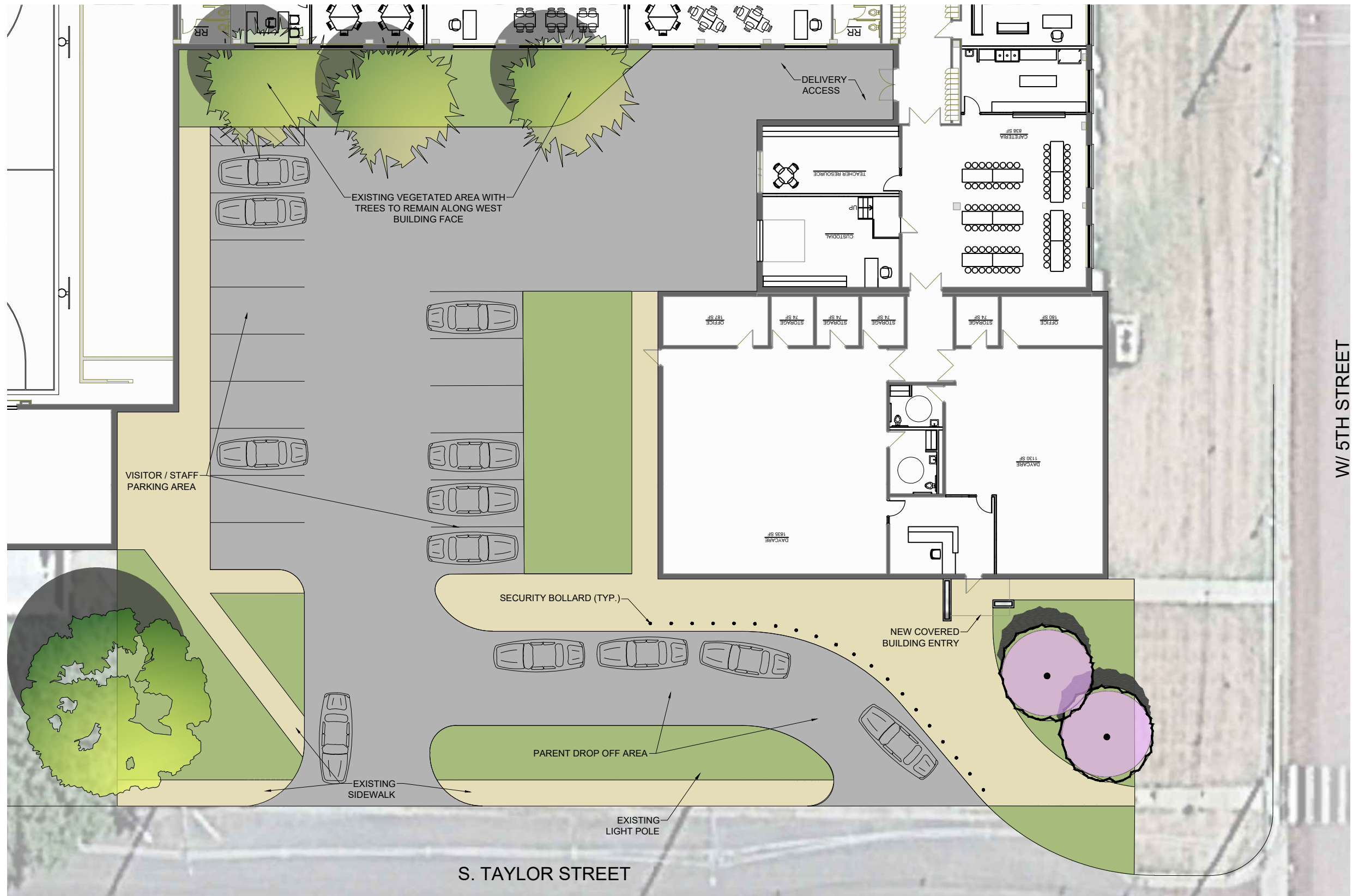
SITE PLAN 1"=10' 0 10'
